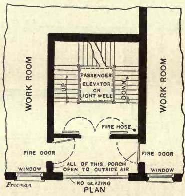
FIG. 16.—TOWER FIRE ESCAPE FOR FACTORIES. PHILADELPHIA TYPE.
