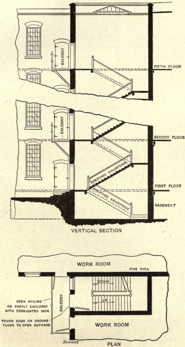
FIG. 15.—BALCONY STAIR TOWER AND FIRE ESCAPE FOR FACTORIES. PHILADELPHIA TYPE.
